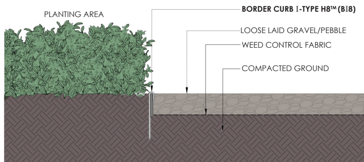
TYPICAL INSTALLATION BORDER CURB I-TYPE H8™ (BI8) WITH GRAVEL
